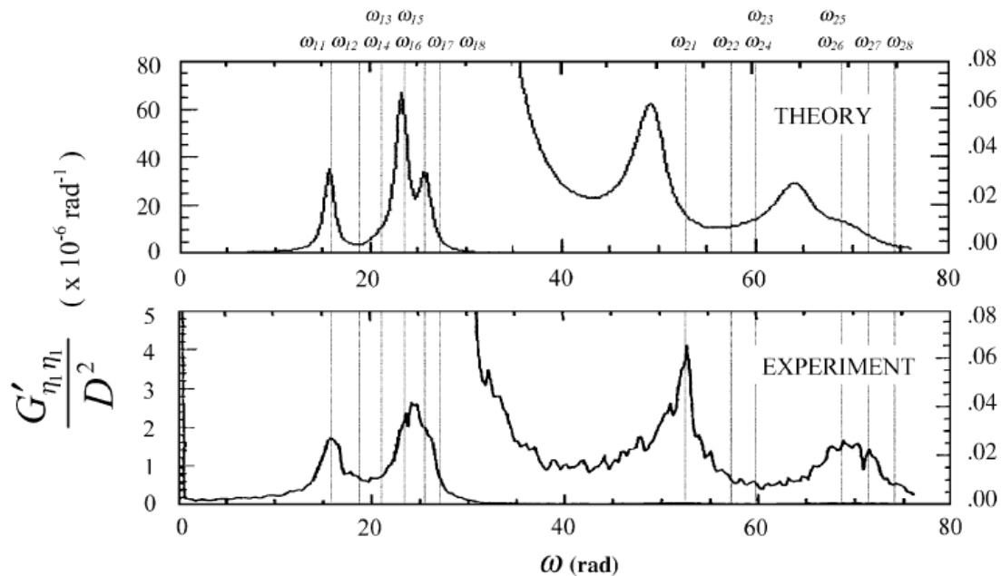
Figure 6: Comparison of theoretical and experimental power spectral densities of mid-cylinder displacements in radial direction in the four-cylinder system [68].
