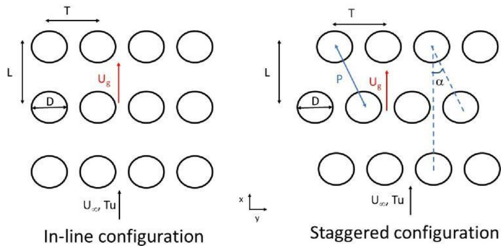
Figure 16: General configurations of the flow through tube arrays, (left) in-inline configuration, (right) staggered configuration, inspired from [16].
