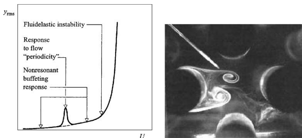
Figure 14: Idealized response with increasing flow reduced-velocity of a cylinder from [3] (left) and downstream vortices of a cylinder [4] (right).
