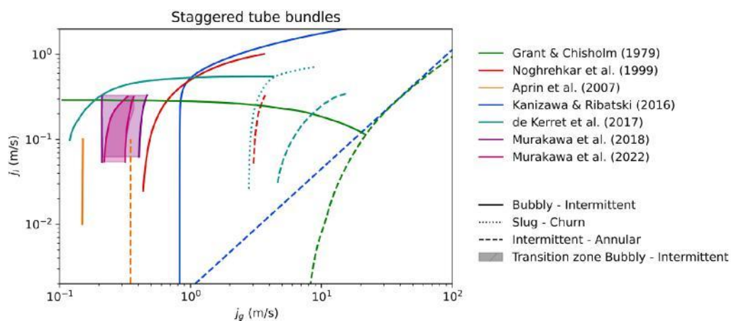
Figure 25: Flow regime map for air-water flow across a triangular tube bundle based on available data from literature.
