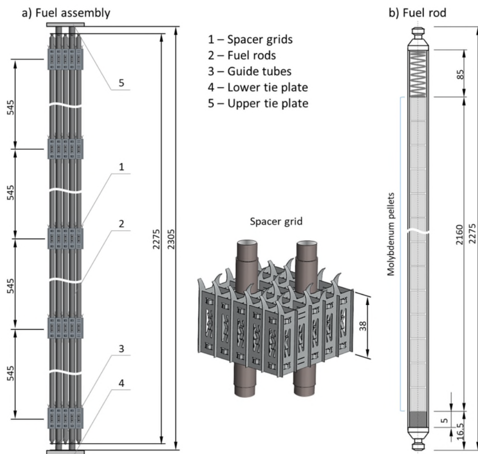
Figure 4: Overview of 5x5 test bundle
