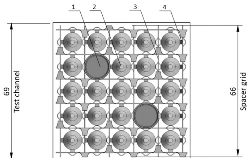
Figure 2: Test bundle and test channel cross-section
